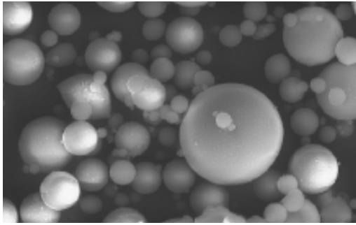
Micrograph of Cholla Fly Ash particles
